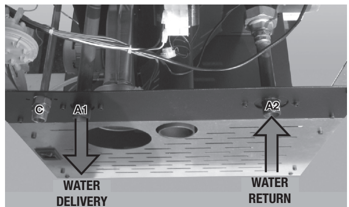
Diagram connection kit without hot water thermostove
