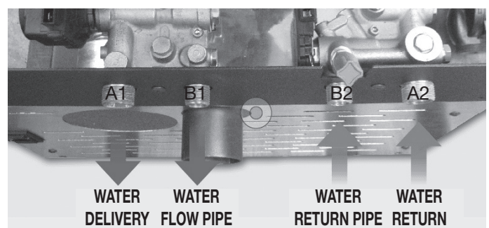
Connection diagram for thermostove equipped with kit for domestic hot water production
